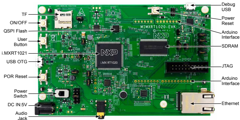
Figure 1: Front side of MIMXRT1020-EVK
