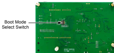
Figure 2: Back side of MIMXRT1020-EVK
