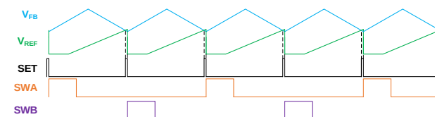
Figure 4: Dual-Phase Interleaving Mode
