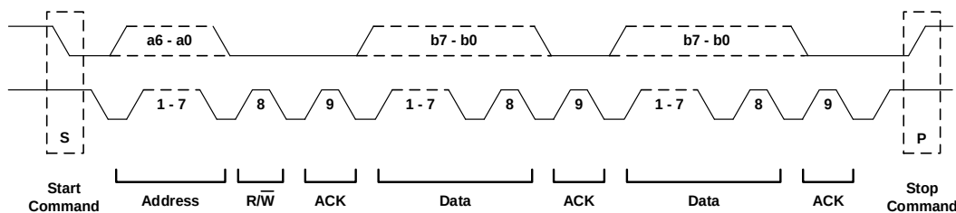
Figure 8: Complete Data Transfer
