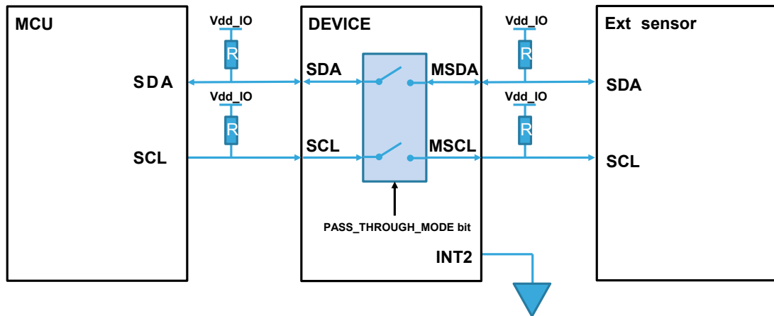
Figure 18. Pass-through feature
