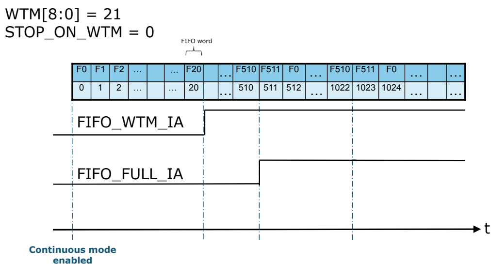
Figure 25. FIFO threshold (STOP_ON_WTM = 0)
