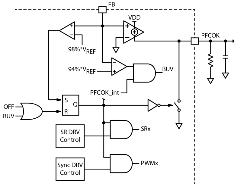
Figure 37. PFCOK Schematic
