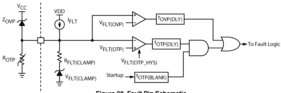
Figure 38. Fault Pin Schematic
