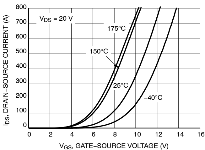
Figure 5. Transfer Characteristic
