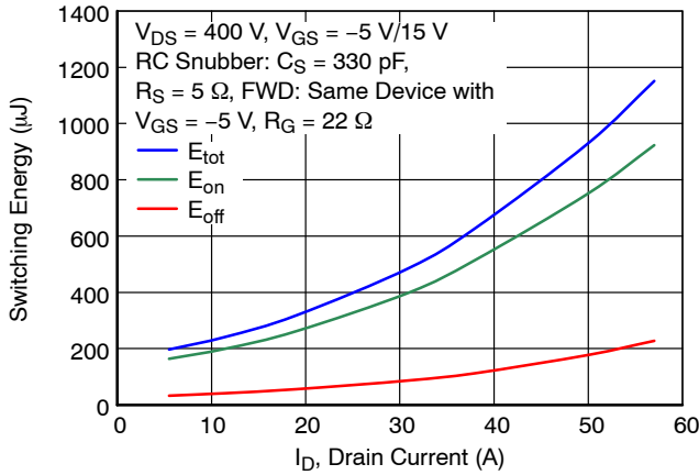
Figure 19. Clamped Inductive Switching Energy vs. Drain Current at T_J = 25\text{ }^\circ\text{C} , Turn-on R_{G\_EXT} = 1.8\ \Omega , and Turn-off R_{G\_EXT} = 22\ \Omega
