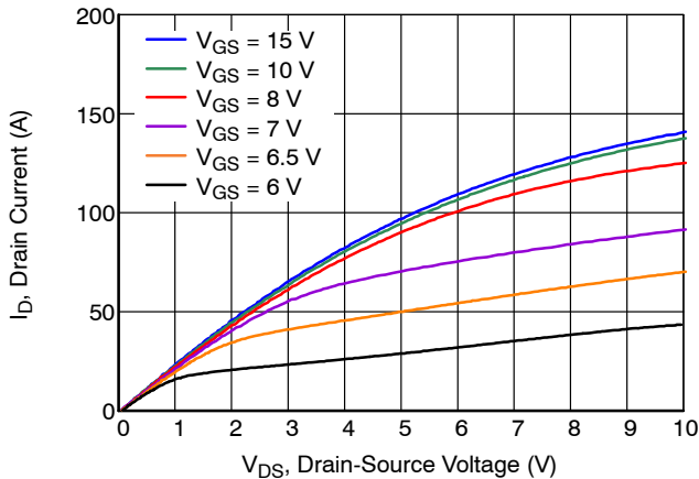
Figure 3. Typical Output Characteristics at T_J = 175\text{ }^\circ\text{C} , t_p < 250\ \mu\text{s}
