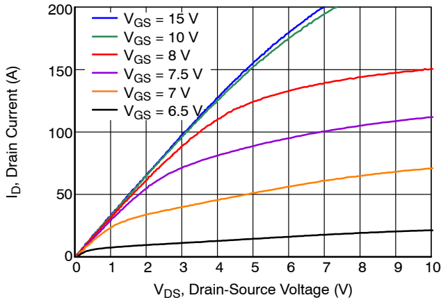
Figure 1. Typical Output Characteristics at T_J = -55\text{ }^\circ\text{C} , t_p < 250\ \mu\text{s}
