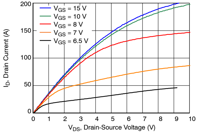
Figure 2. Typical Output Characteristics at T_J = 25\text{ }^\circ\text{C} , t_p < 250\ \mu\text{s}
