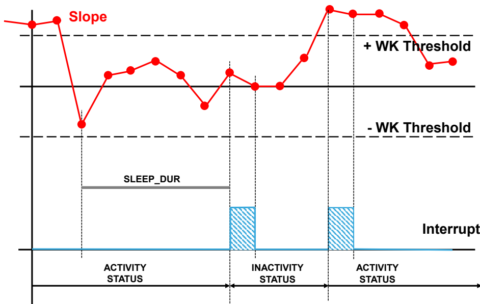
Figure 6. Activity/inactivity recognition (using the slope filter)
