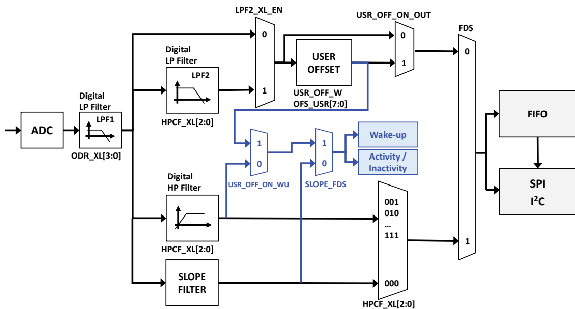
Figure 2. Accelerometer filtering chain
