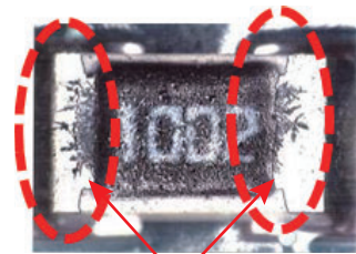
Sulfurated Ag needle crystal
