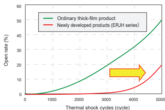
Extended solder life by suppressing crack progress
