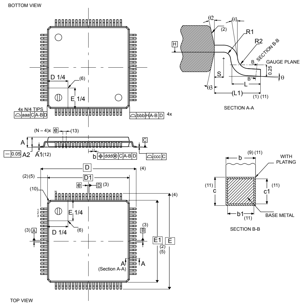
Figure 54. LQFP80 - Outline (15.)
