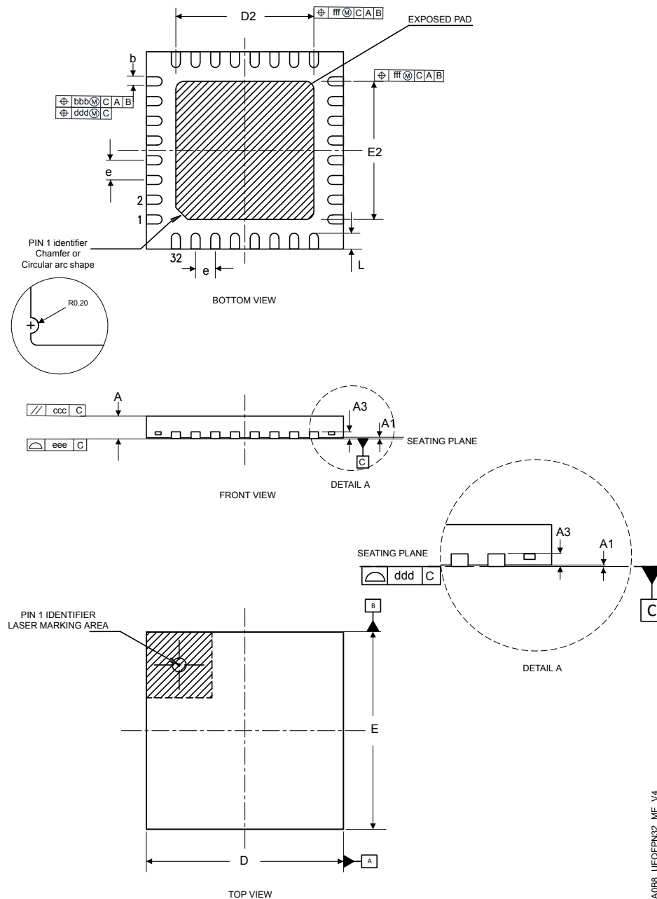
Figure 47. UFQFPN32 - Outline
